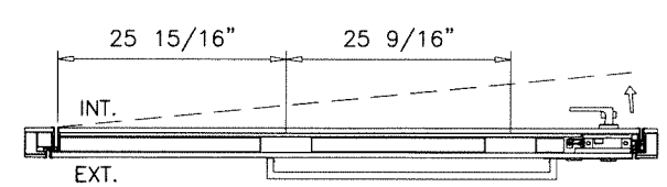
TYPICAL ELEVATION (INSWING PIVOT DOOR)
